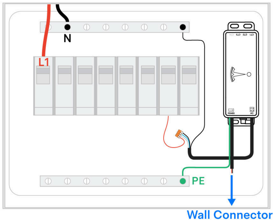
Figure 6. RS-485 Protective Earth Conductor Connected to Distribution Board Equipment Ground Board (Single Phase Example)
